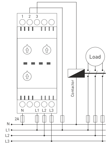
Connection Diagram for FKT-06/06F/06PF
