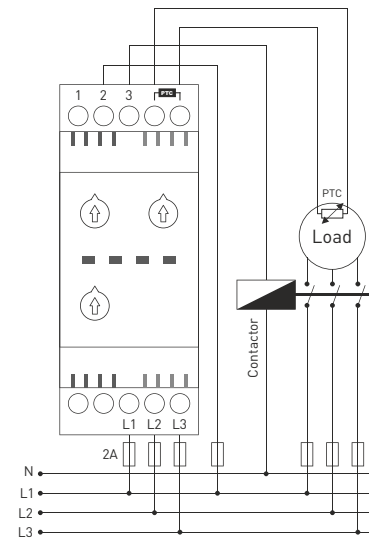
Connection Diagram for FKT-06/06F/06PF
